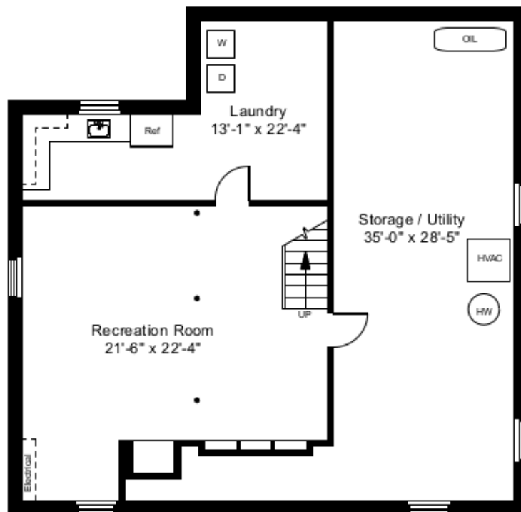
Lower Level Plan Ceiling Height = 7'-3"
