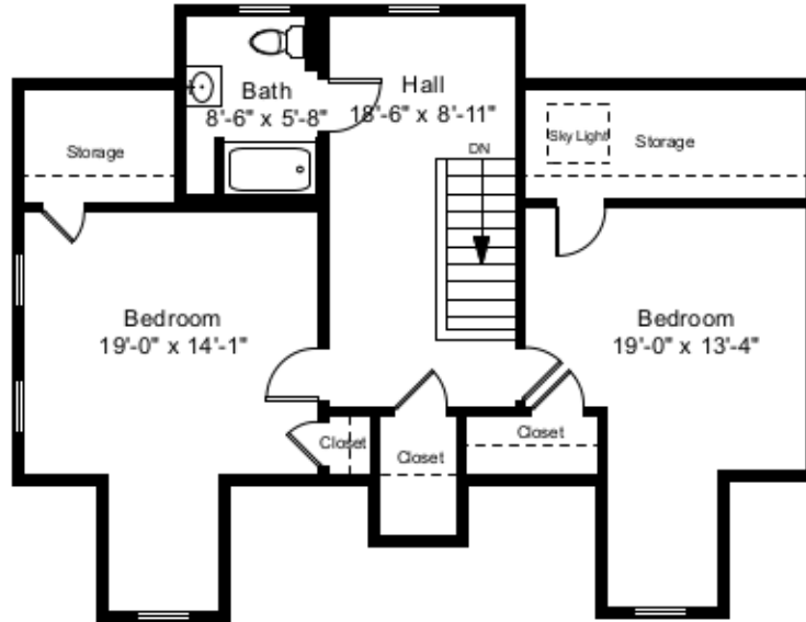
Third Floor Plan Ceiling Height = 6'-9"
